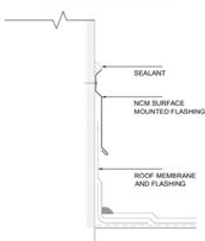
SURFACE MOUNTED FLASHING (TYP. DETAIL)
