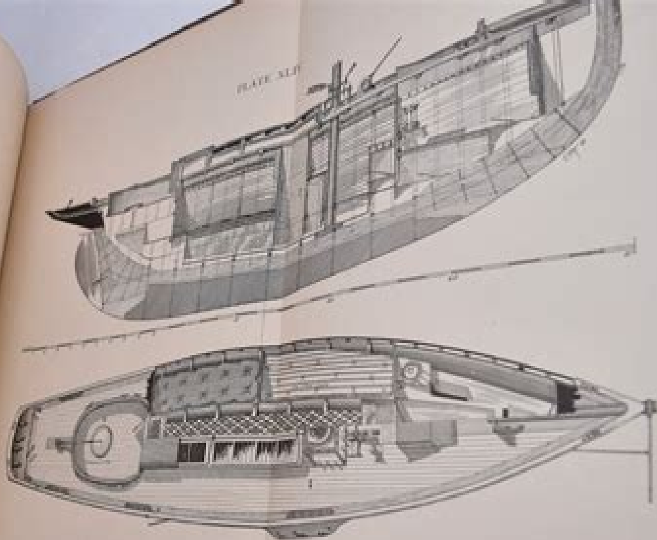
THE USS ALBATROSS—CARRY AND DECK PLAN.
