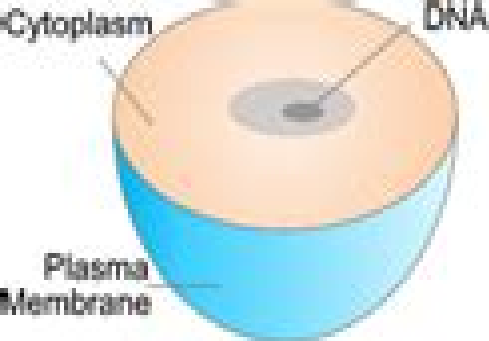
Ancestral prokaryote
