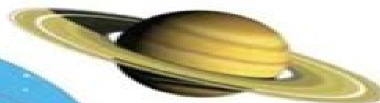
Saturn's rings
