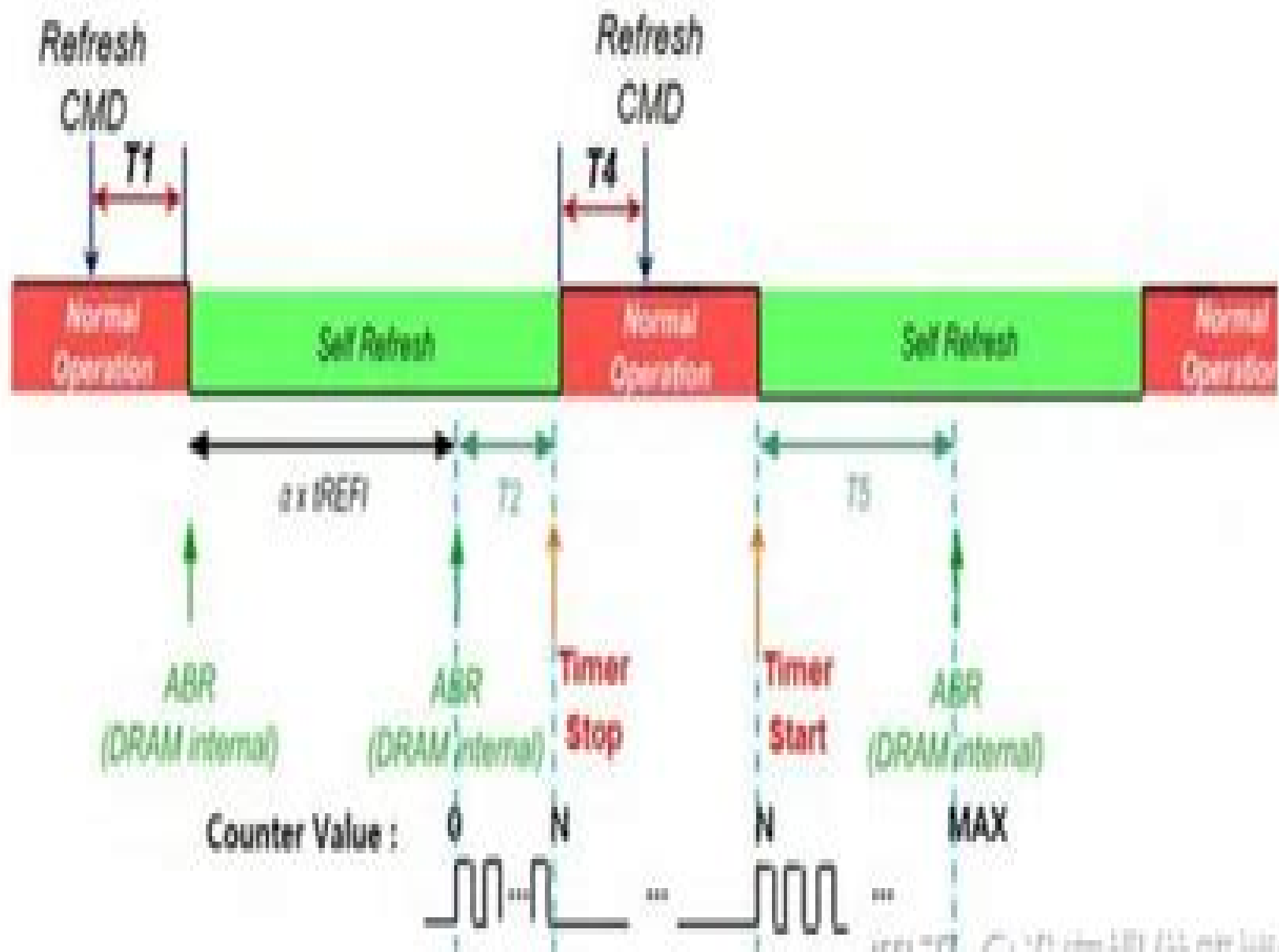
Figure 139 — Optimized Refresh Operation
