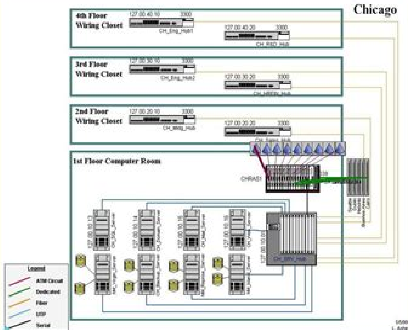
Figure 12-1 Network configuration diagram (source: netViz).
