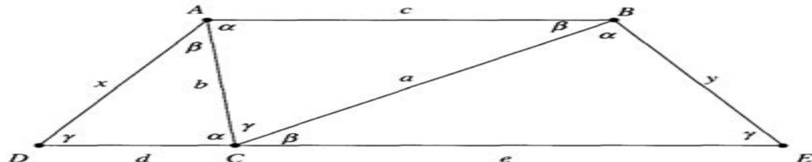
FIGURE 1: Isosceles trapezium
