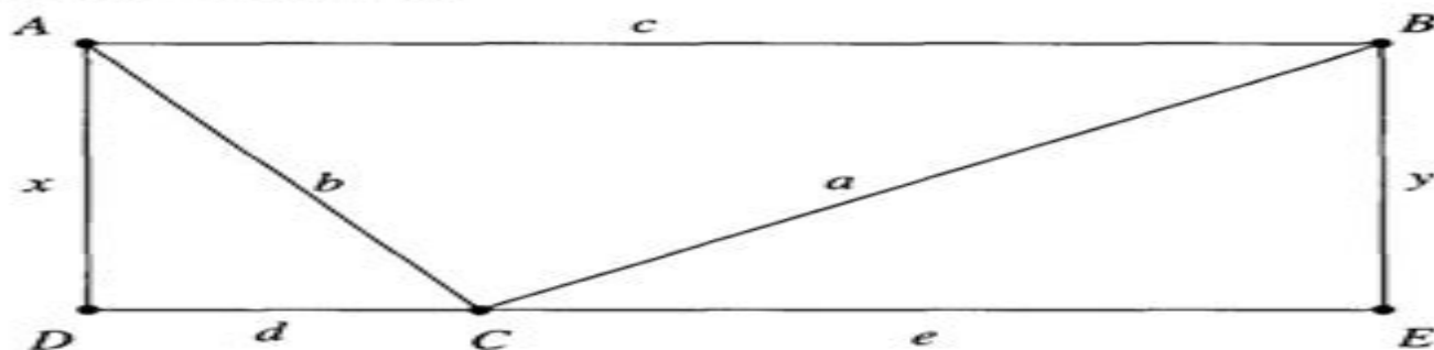
FIGURE 2: 'Rectangular' trapezium
