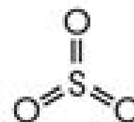
Sulfur trioxide
