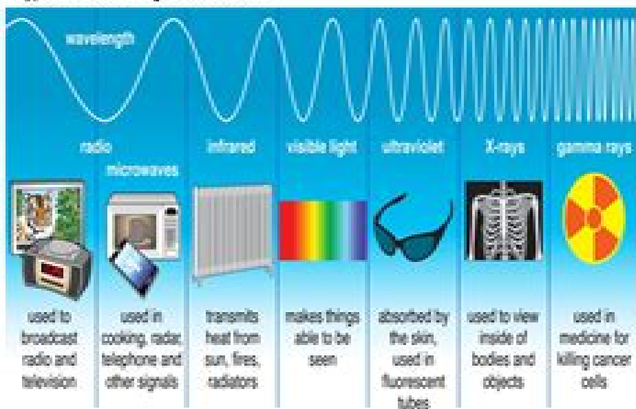
Types of Electromagnetic Radiation
