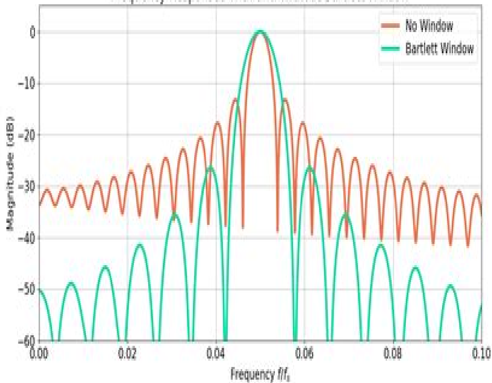
Frequency Responses With and Without Bartlett Window
