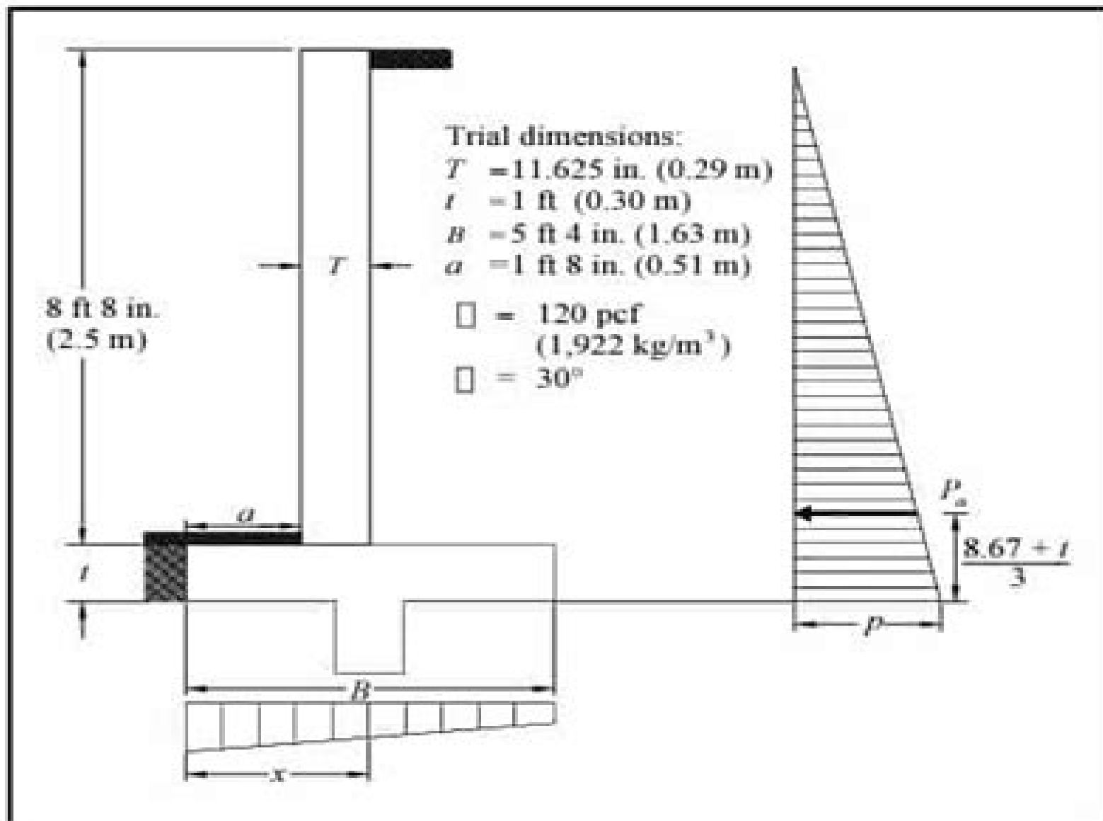
Figure 2—Reinforced Cantilever Retaining Wall Design Example
