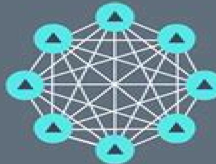
HOPFIELD NETWORK
