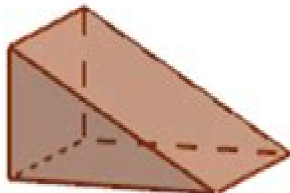
Triangular prism
