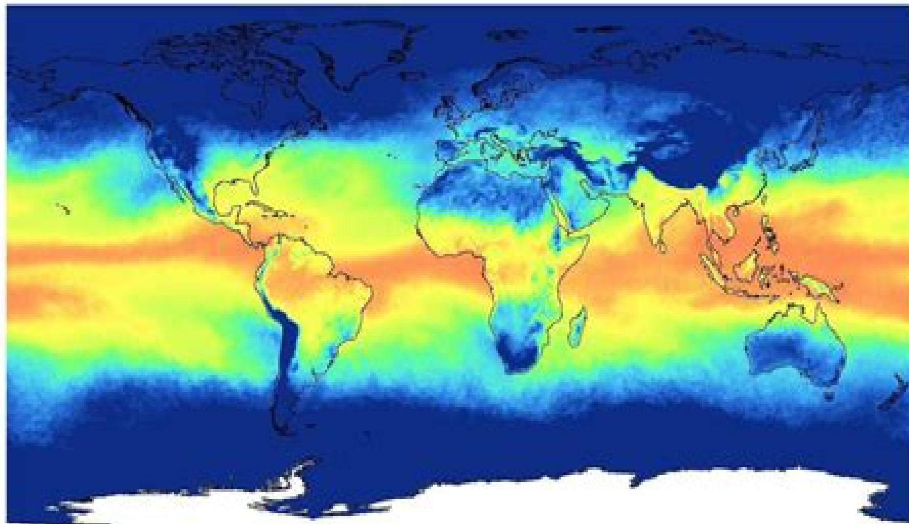
AIRS TOTAL PRECIPITABLE WATER VAPOR (mm), May 2009
