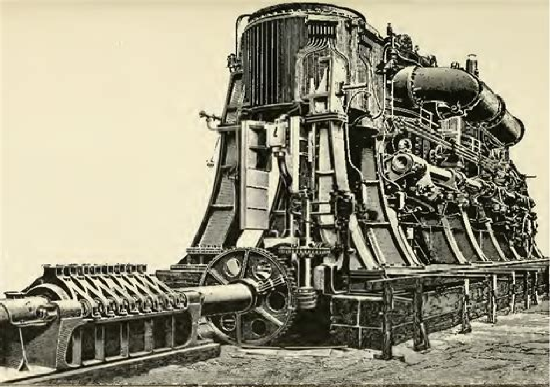
FIG. 15.—END VIEW OF THE "TERRIBLE'S" ENGINES.
