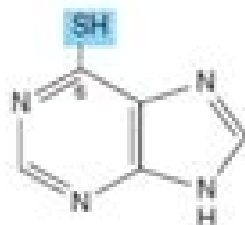
6-Mercaptopurine
