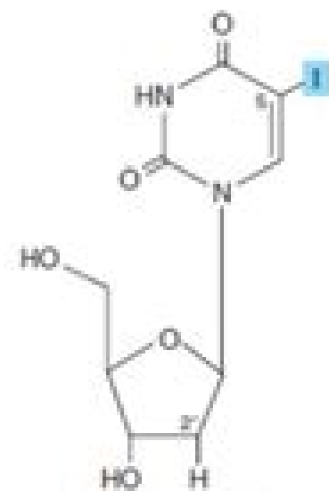
5-Iodo-2'-deoxyuridine
