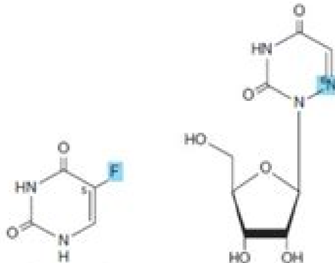
5-Fluorouracil
