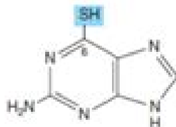
6-Thioguanine
