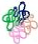
Protein aggregation
