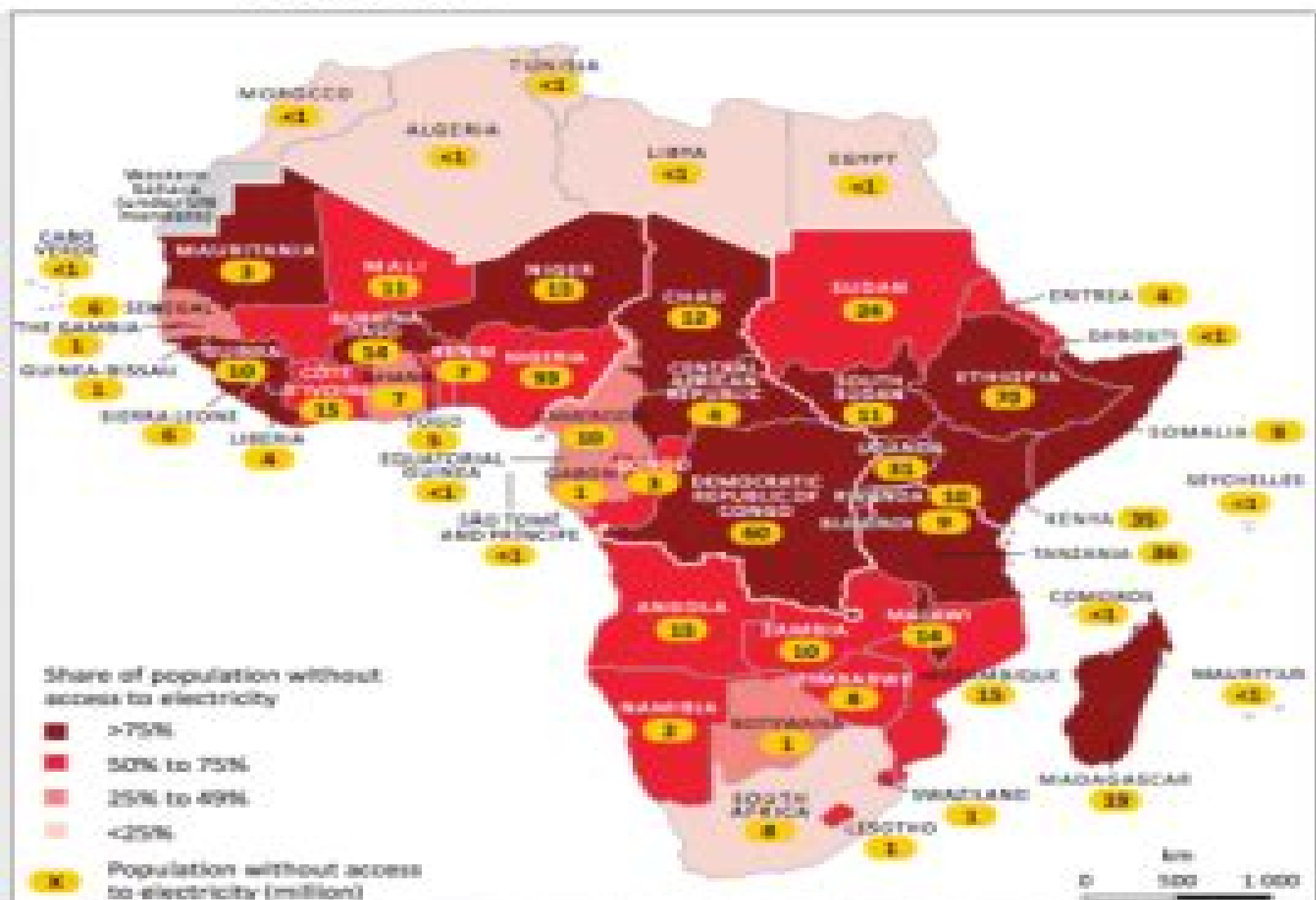
Figure 1.6 — Number and share of people without access to electricity by country, 2012
