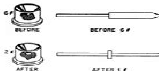
FIG. 4-2. Centering support and pin after modification.
