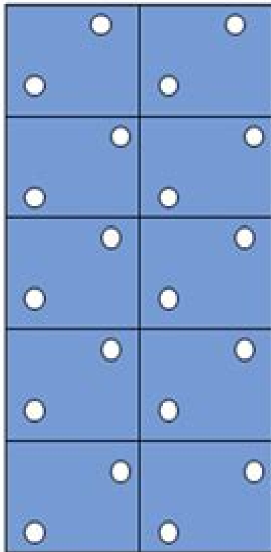
Uniform
