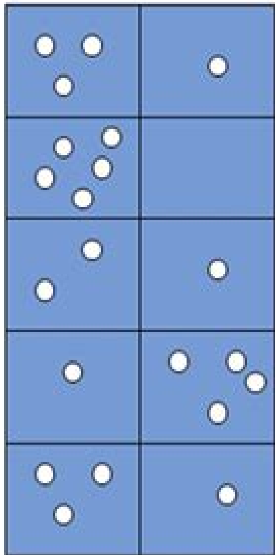
Random
