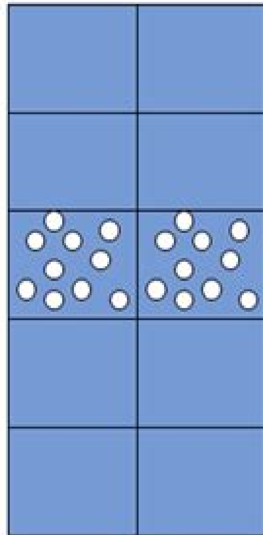
Clustered
