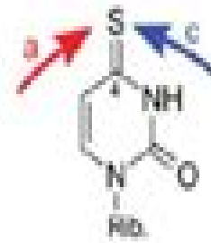
4-thiouridine s 4 U
