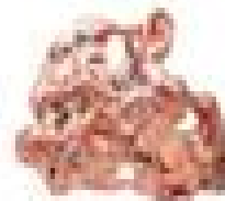
native copper
