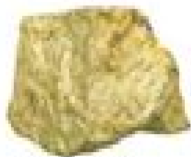
chalcopyrite
