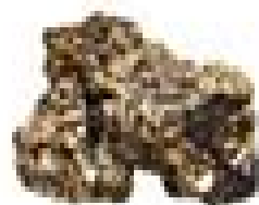
pyrite
