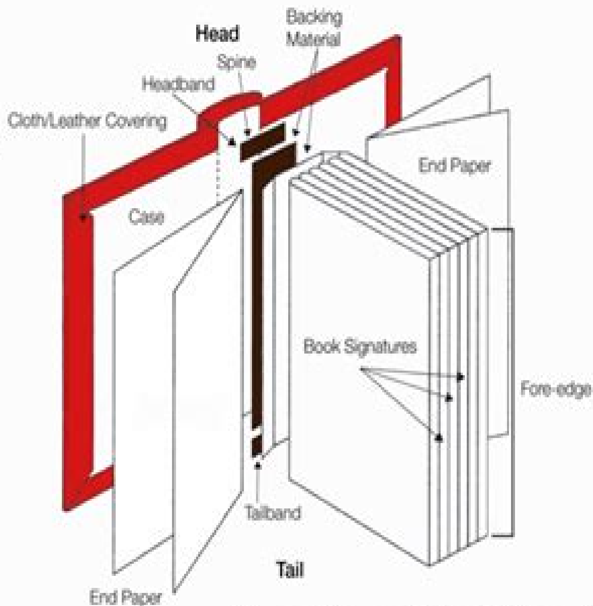
Case Bound Book Construction
