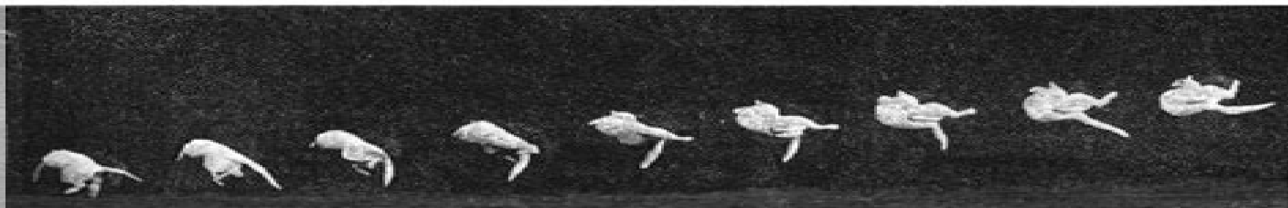
FIG. 2.—End view of a falling cat. (The series runs from right to left.)
