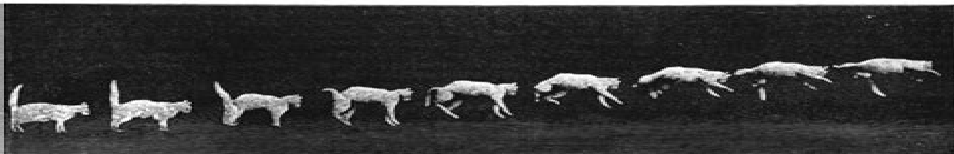
FIG. 1.—Side view of a falling cat. (The series runs from right to left.)
