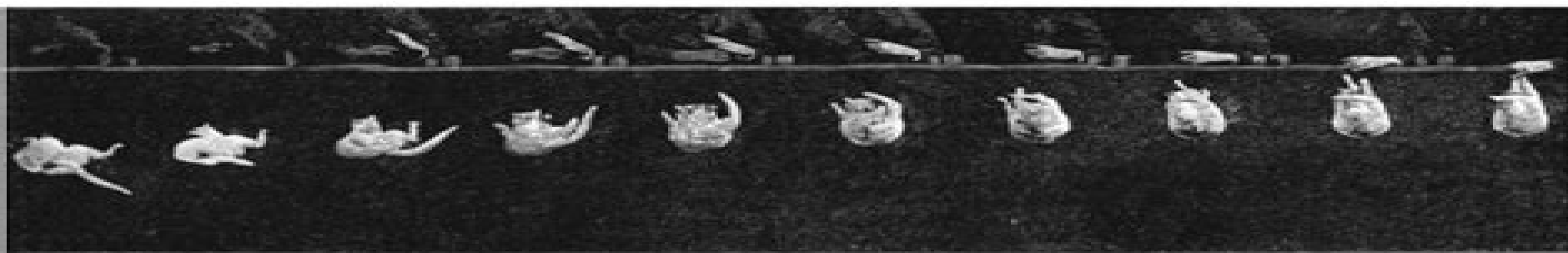
FIG. 1.—Side view of a falling cat. (The series runs from right to left.)
