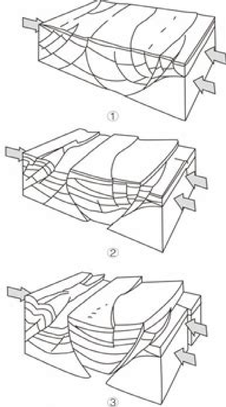
(c) Tectonic evolution stages of geological body
