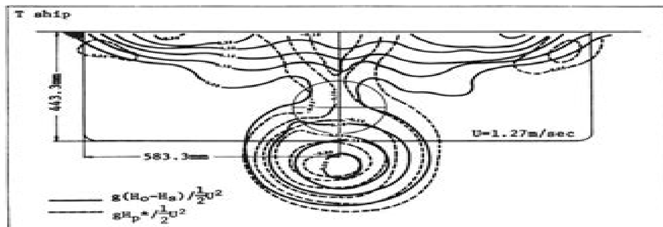
MEASUREMENT SECTION 0.5L pp behind A.P.
