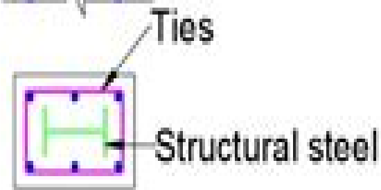
Composite Column
