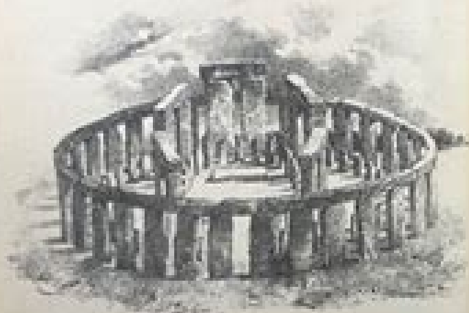
STONEHENGE RESTORED
