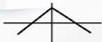
Short Straddle
