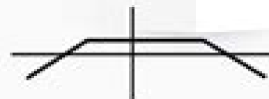
Short Straddle
