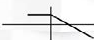
Short Call
