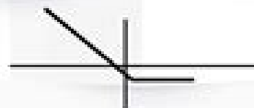
Long Put
