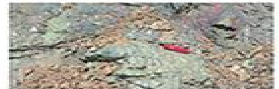
Gabbro, Timbucktoo, Sierra Nevada, California
