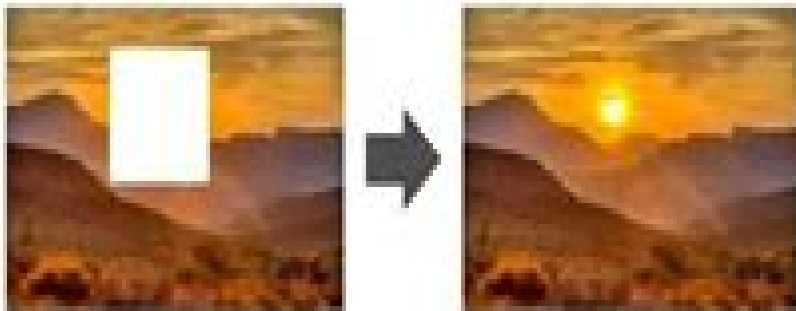
Image Inpainting
