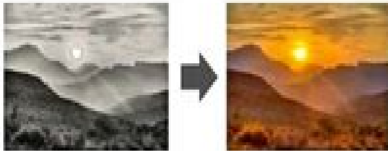
Colourization
