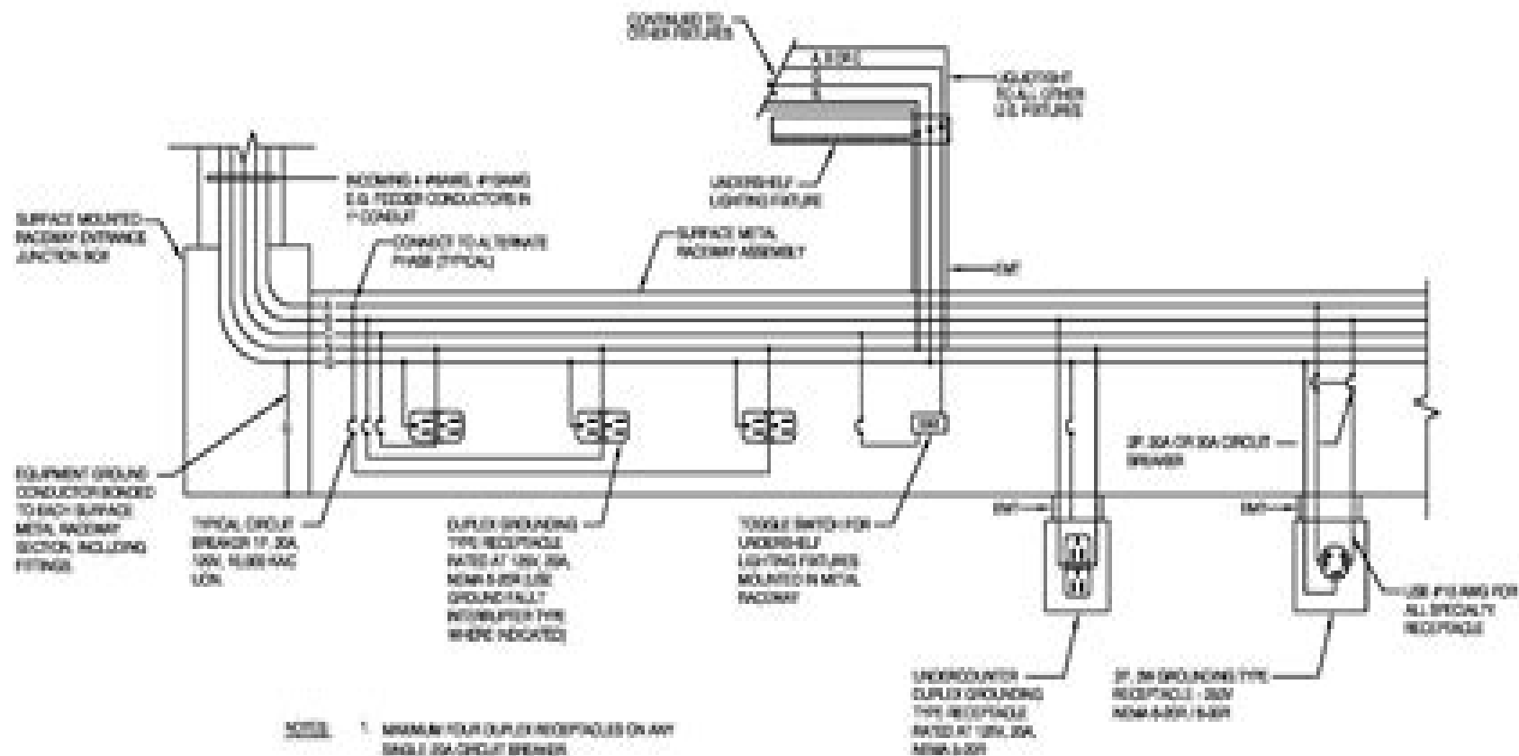
SURFACE METAL RACEWAY WIRING DETAIL NO SCALE
