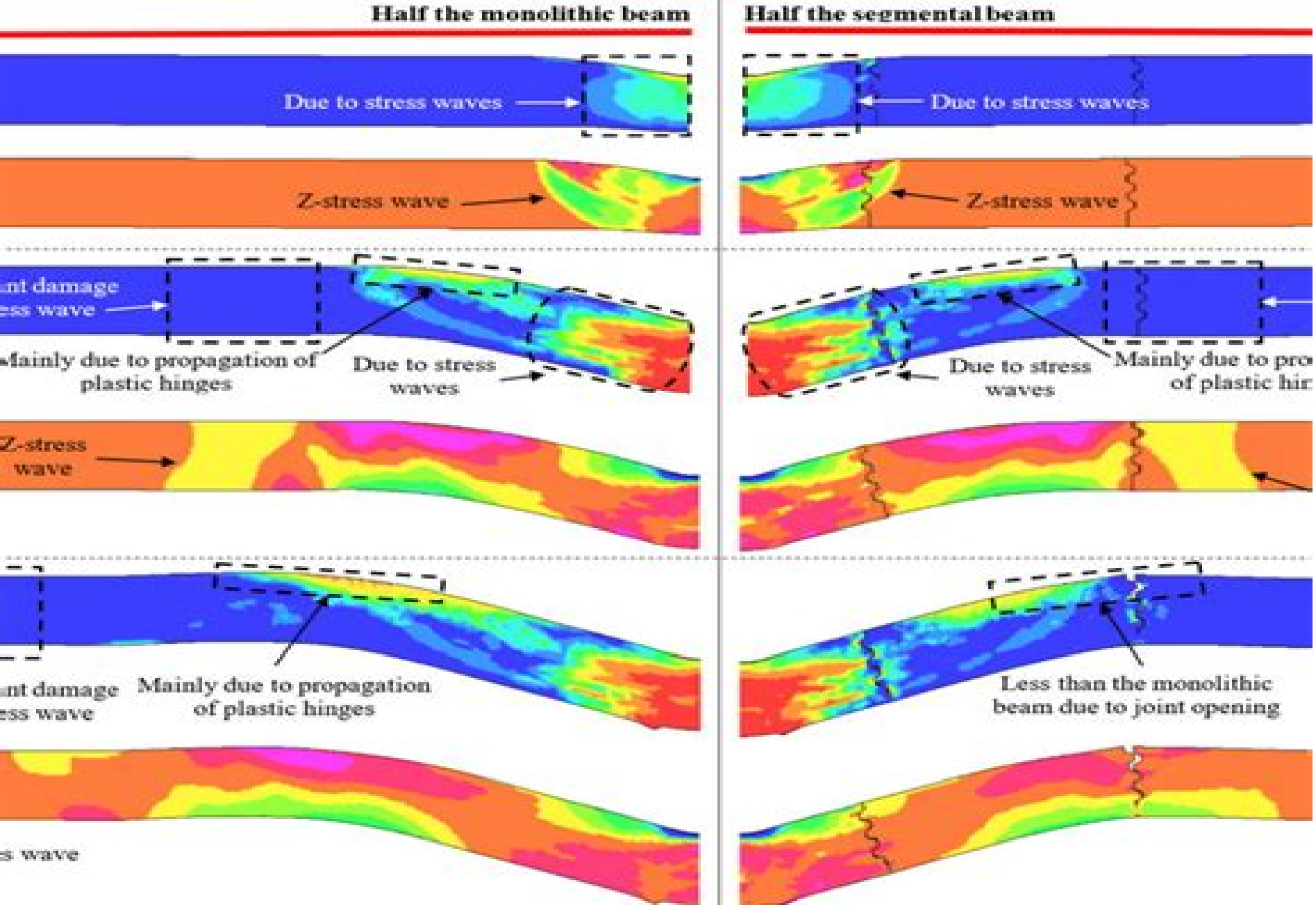
Fig. 11. Propagation of blast-induced stress waves (half beam)
