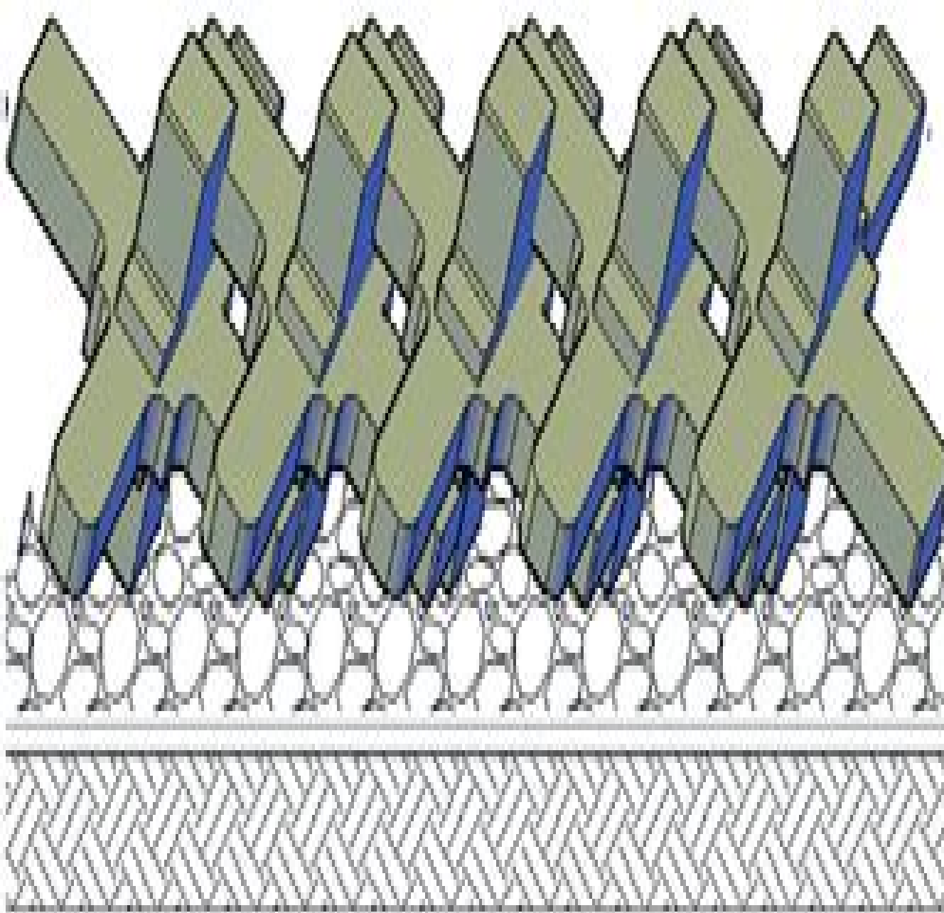
FIGURE 1: Geometric shape of six-legged elements and an instance of A. Jacks armors' interlock
