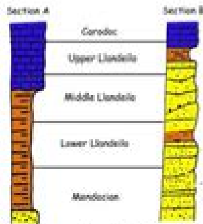
Chronostratigraphic Correlation
