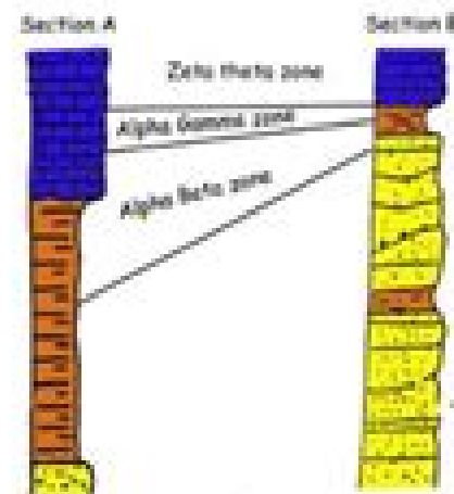
Biostratigraphic Correlation
