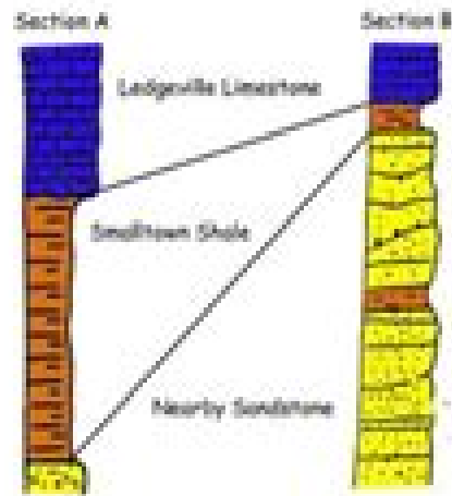
Lithostratigraphic Correlation
