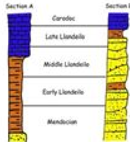
Geochronologic Correlation
