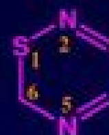
6H-1,2,5-thiadiazine
