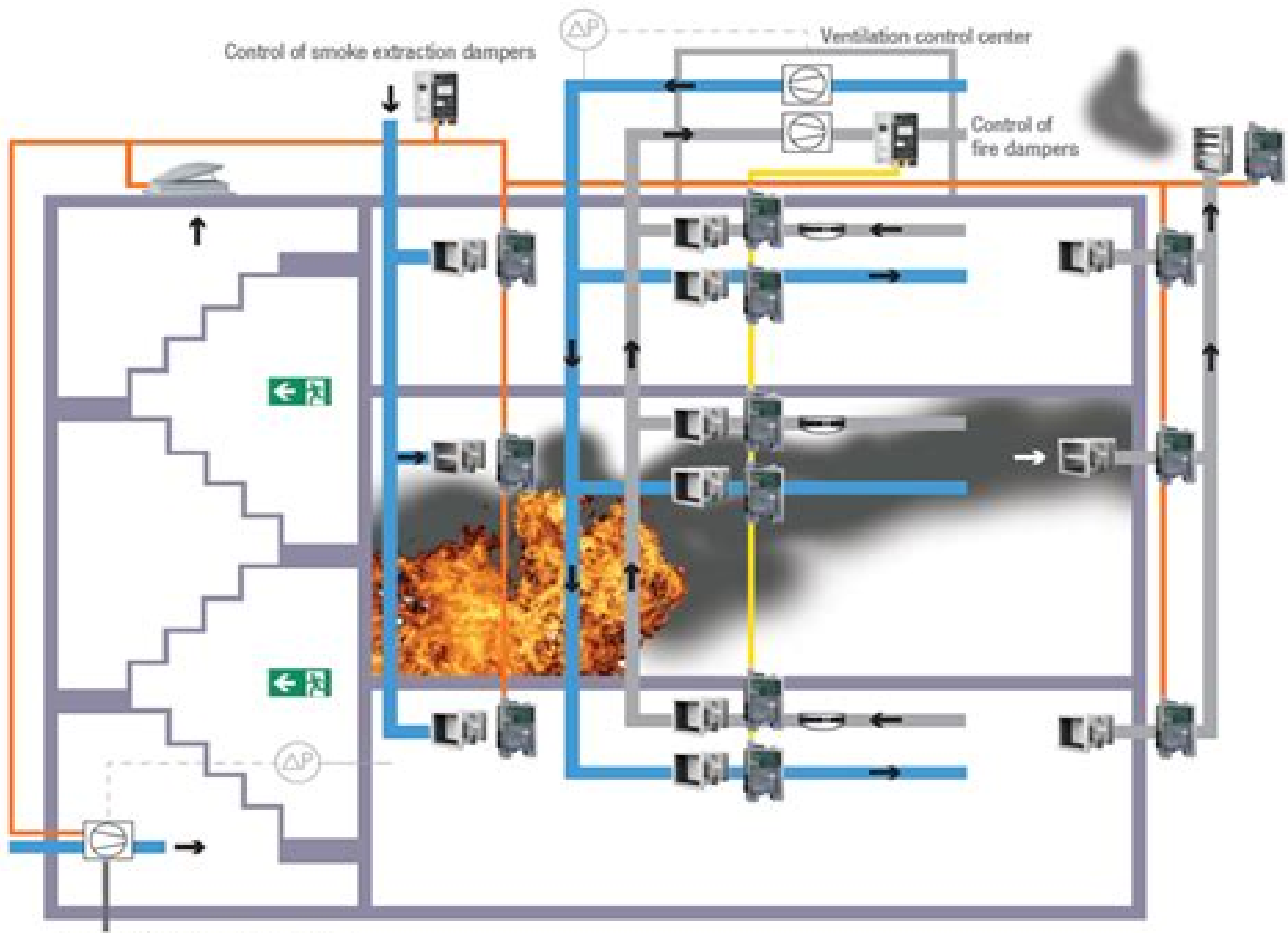
Smoke protection pressure system Smoke and heat exhaust ventilation system
