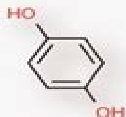
Hydroquinone
