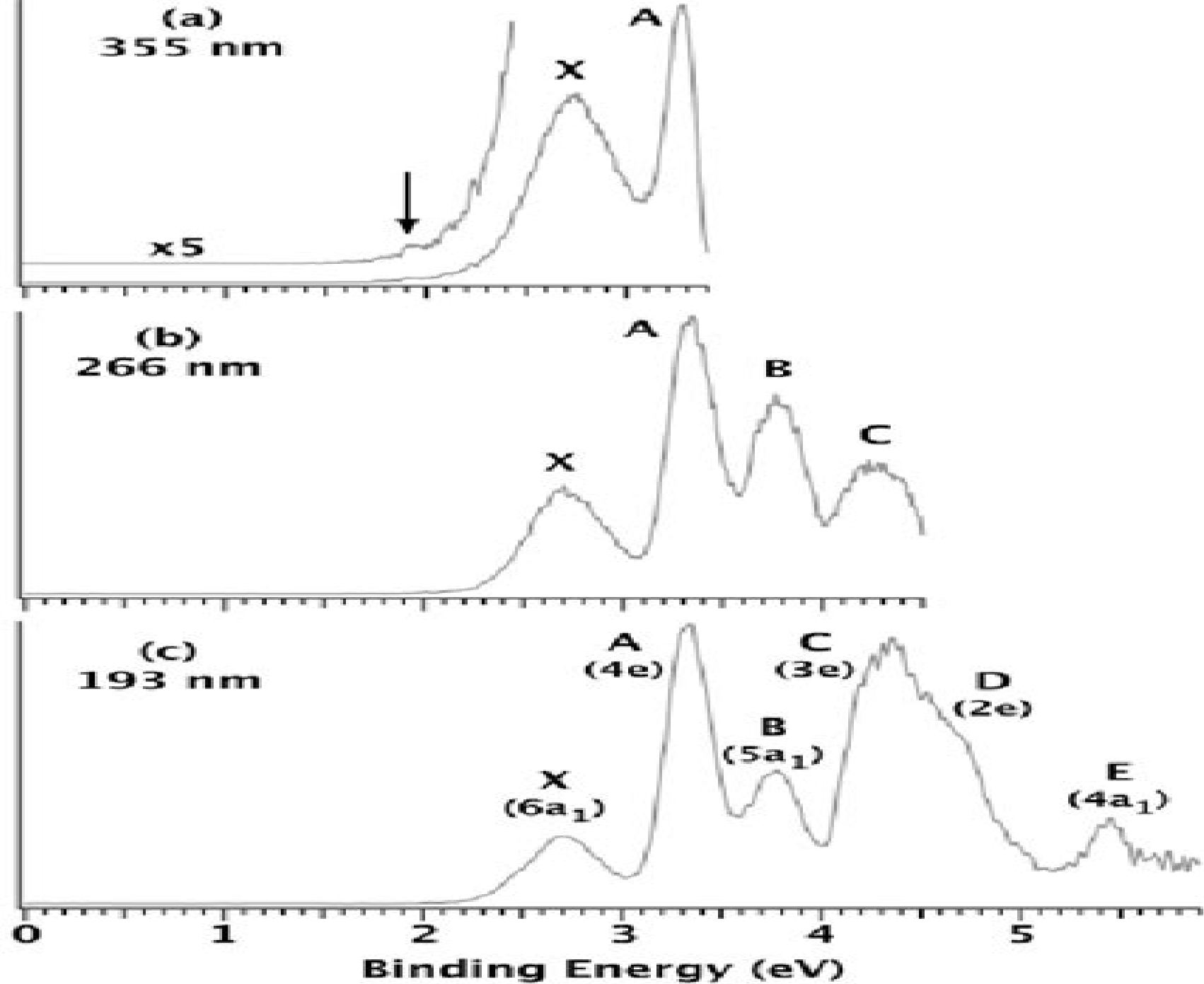
Fig. 1. Photoelectron spectra of Al-NTF at (a) 355 nm (3.49 eV), (b) 266 nm (4.66 eV), and (c) 193 nm (6.42 eV).
