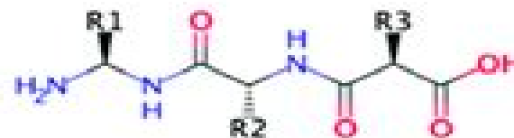
Retro-inverse Peptide Regular End-Groups
