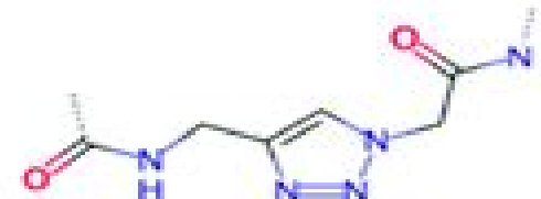
triazole peptide
