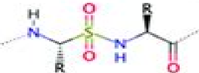
carbonyl replacement
