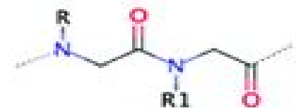
peptoids
