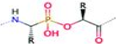
phosphonopeptide
