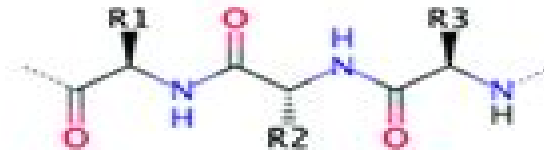
Retro-inverse Peptide
