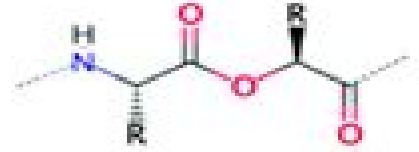
depsipeptide
