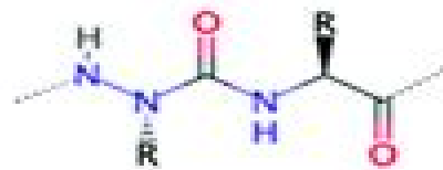
azapeptide
