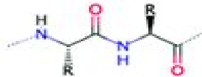
Normal Peptide
