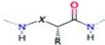
backbone extension
