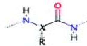
\alpha replacement
