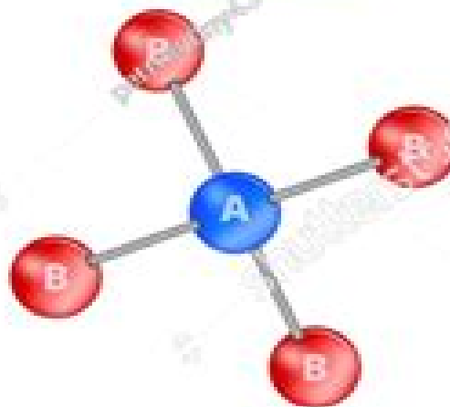
Tetrahedral
