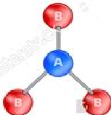
Trigonal Planar
