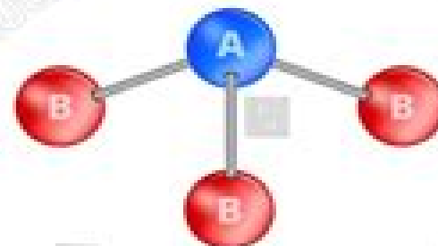
Trigonal Pyramidal
