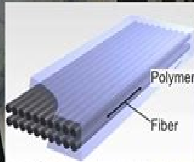
Carbon-FRP (CFRP) plates bonded to concrete surface with adhesive
