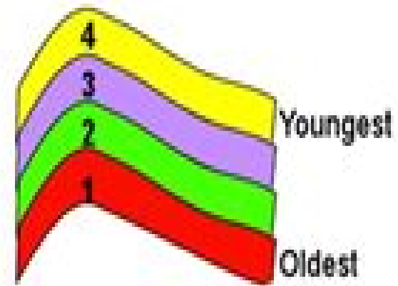
Law of Original Horizontality (originally like figure to the right)
