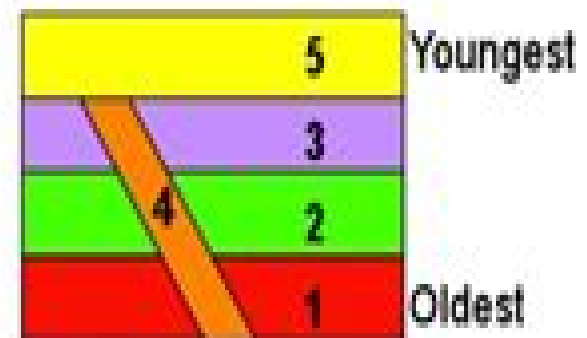
Cross-Cutting Relationship
