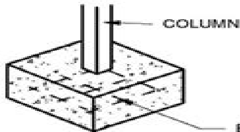
ISOLATED CONCRETE FOOTING (SHALLOW FOUNDATION)
