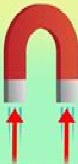
ELECTRO- MAGNETISM
