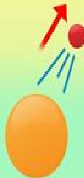
WEAK FORCE
