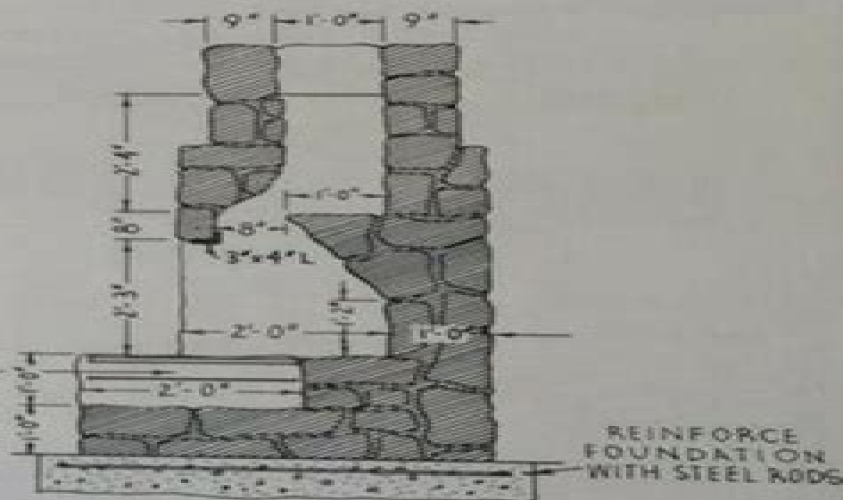
CROSS SECTION
