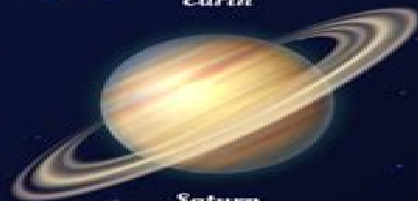
Saturn
