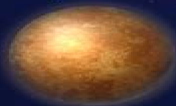
Mercury
