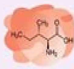
Isoleucine
