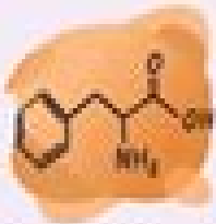
Phenylalanine
