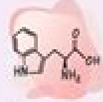
Tryptophan
