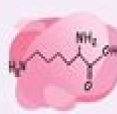
Lysine
