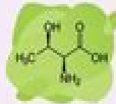
Threonine
