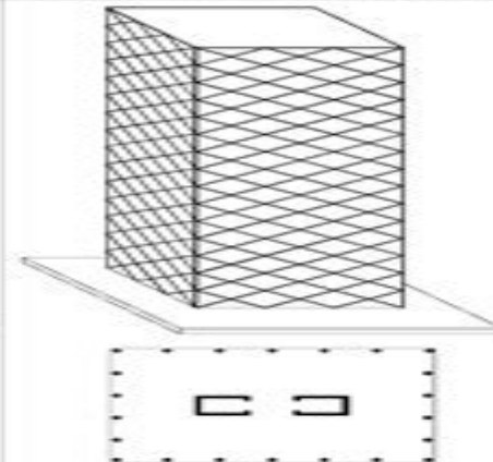
Diagrid-Tube System
