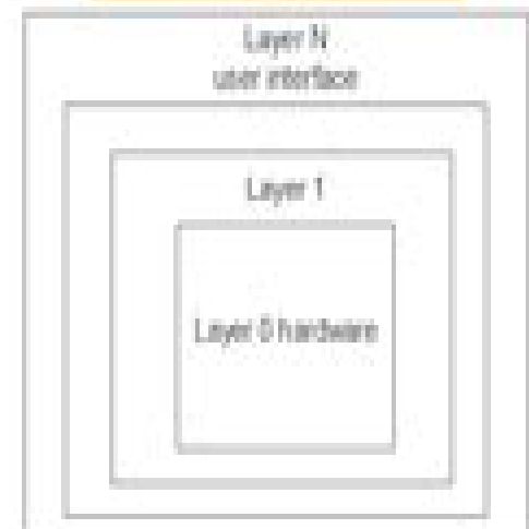
Layered - structure
