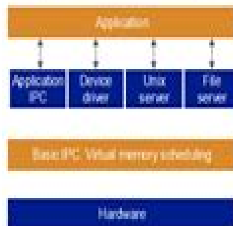
Micro-kernel structure
